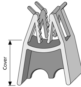
Fix: 30-40-50 mm
